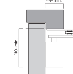
Fig.66 Parallel arm push side mount
