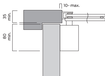
Fig.1 Door mount pull side
