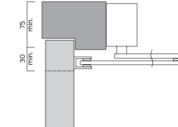
Fig.61 Transom mount push side
